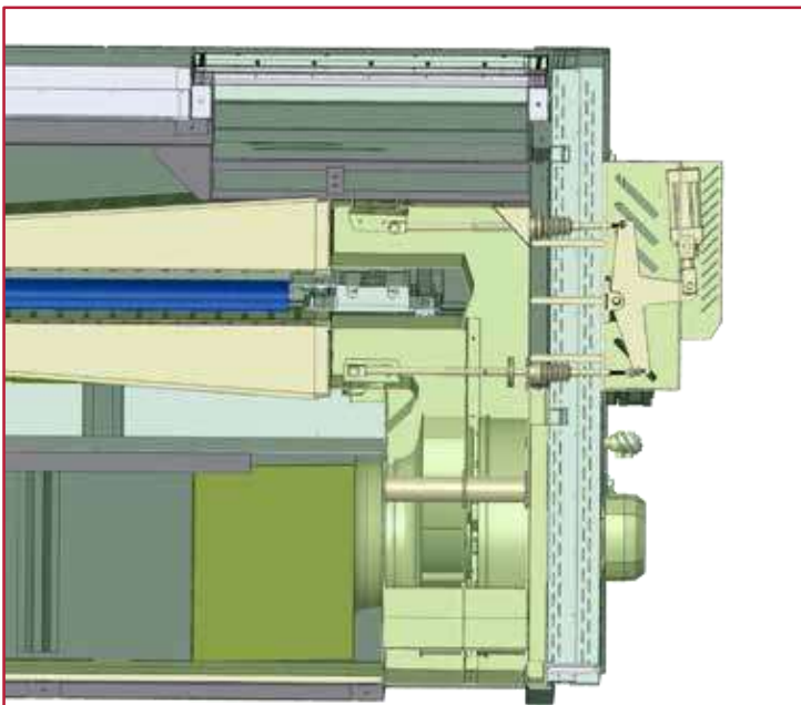
Pistonlu Tip Klepe Sistemi / Piston Type Flap System For automatic control of air transfer inside the suction filters
