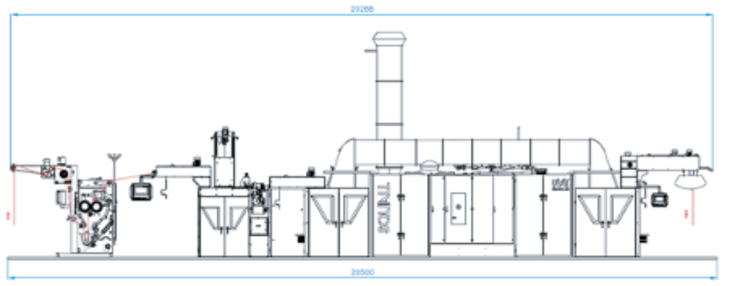
ÖN KURUTMALI/ WITH PRE-DRYING
